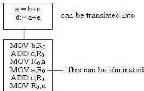
Figure 5.2 Code Translation
