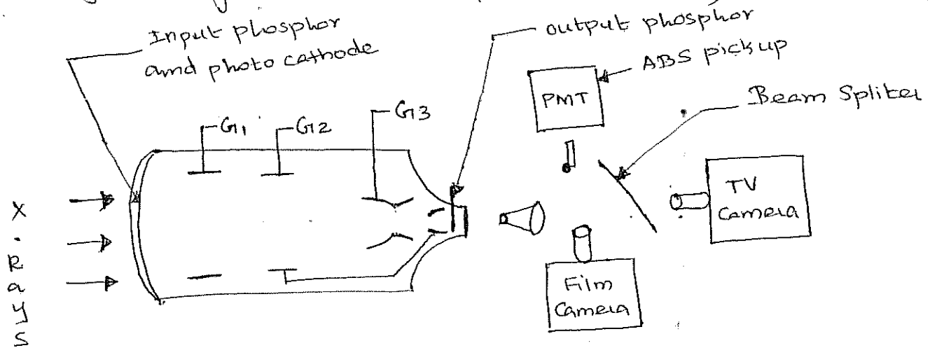
Fig: Image intensifiers (Fluoroscopy)
