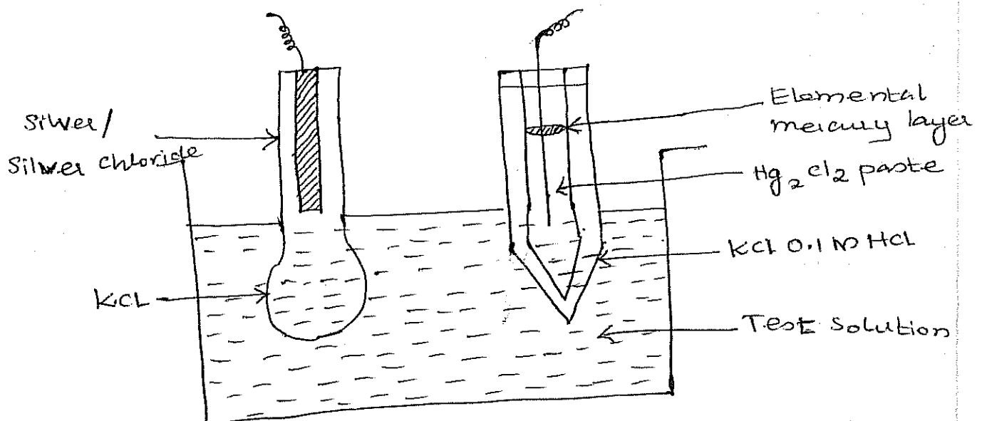
pH Electrode.
