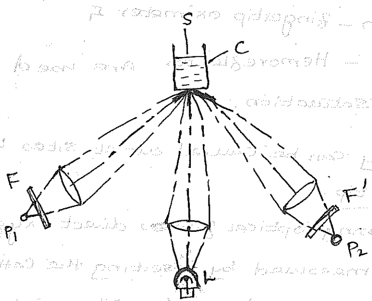
Optical arrangement in reflection oximeter.
