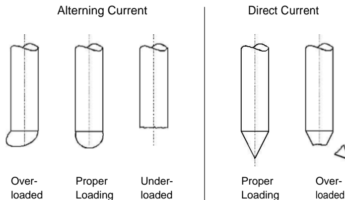
Current Loading of the Tungsten Electrode
