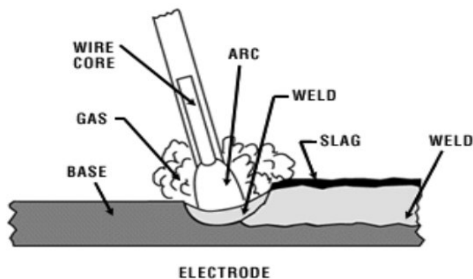
STICK WELDING PROCESS
