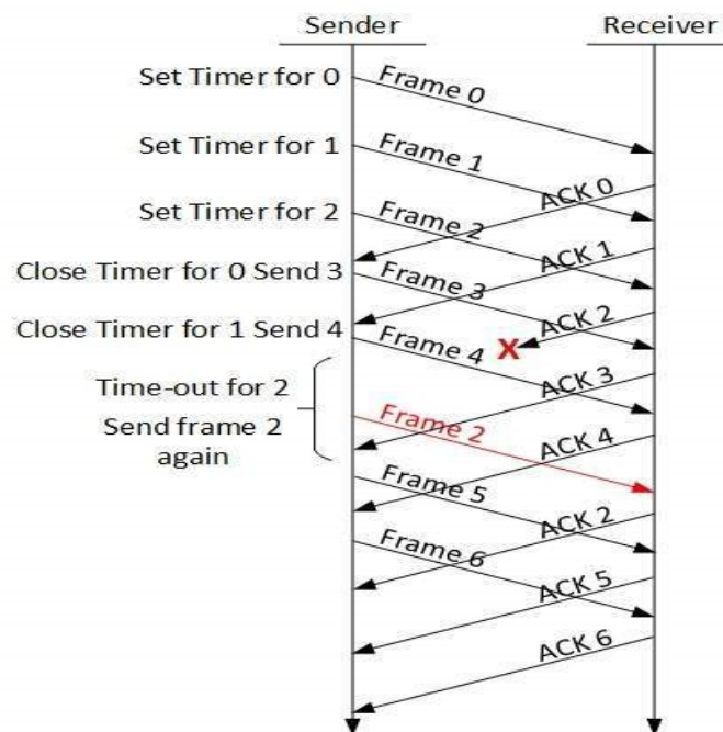
Fig 2.14 Selective-Repeat ARQ
