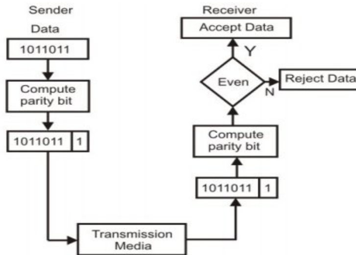
Fig 2.8 Even-parity checking scheme
