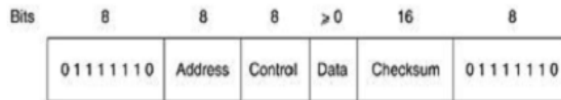
Fig 2.15 High-Level Data Link Control
