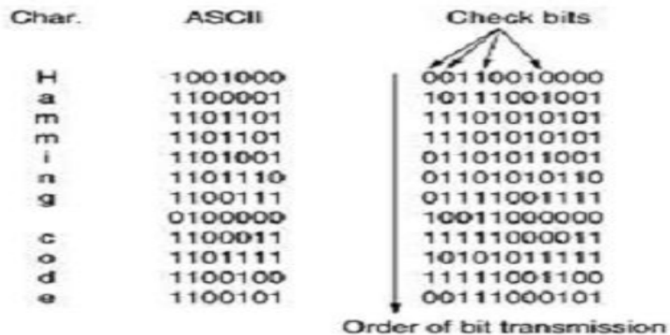
Fig 2.9: Use of a Hamming code to correct burst errors
