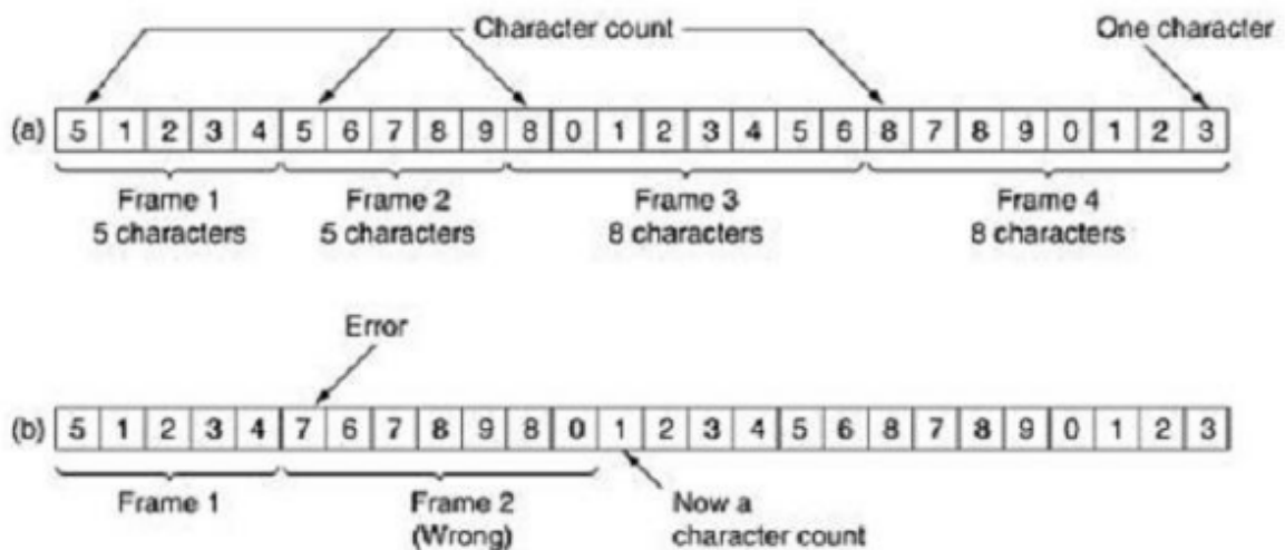
Fig 2.18 Framing
