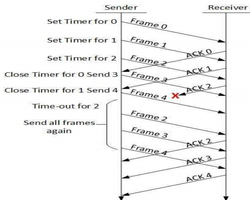
Fig 2.13 Go-Back-N ARQ
